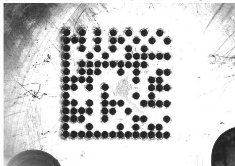
Figure 3.2.3-1 GS1 DataMatrix dot-peened symbol
